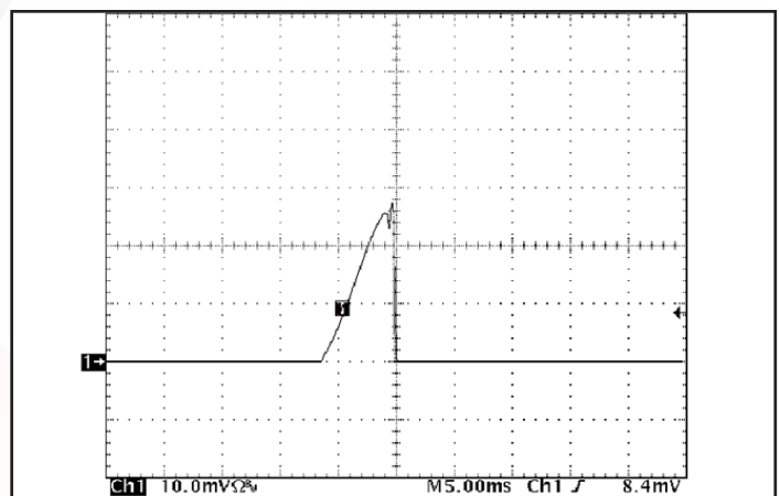
Figure 18: Load current (50A/div) as a function of time (5ms/div) when the converter attempts to turn on into a 10\ \text{m}\Omega short circuit.
