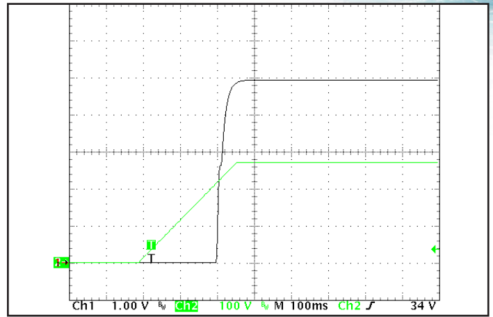
Figure 8: Turn-on transient at full resistive load and zero output capacitance initiated by Vin. ON/OFF Pin previously low. Ch 1: Vout (1V/div). Ch 2: Vin (100V/div).
