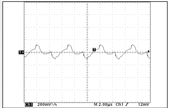
Figure 10: Output voltage ripple, 5Vout, at nominal input voltage and rated load current (200 mV/div). Load capacitance: 1µF ceramic capacitor and 15µF tantalum capacitor. Bandwidth: 10 MHz. See Figure 17.
