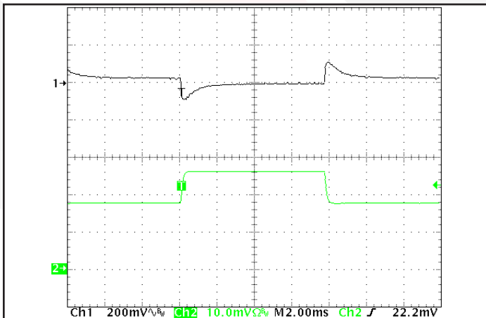
Figure 11: Output voltage response to step-change in load current (50%-75%-50% of Iout(max); dI/dt = 0.1 A/\mu s ). Load cap: 1 µF ceramic and 15 µF tantalum capacitors. Ch 1: Vout (200mV/div), Ch 2: Iout (20A/div).
