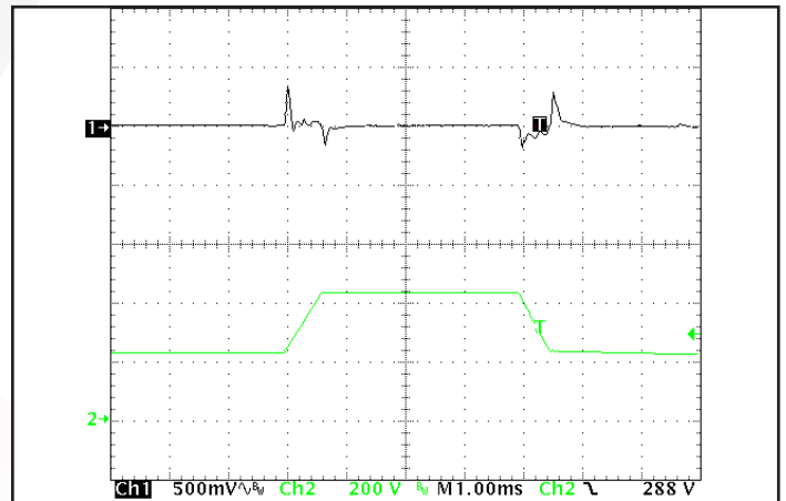
Figure 12: Output voltage response to step-change in input voltage (250V/ms). Load cap: 1µF ceramic and 15µF tantalum capacitors. Ch 1: Vout (500mV/div), Ch 2: Vin (200V/div).
